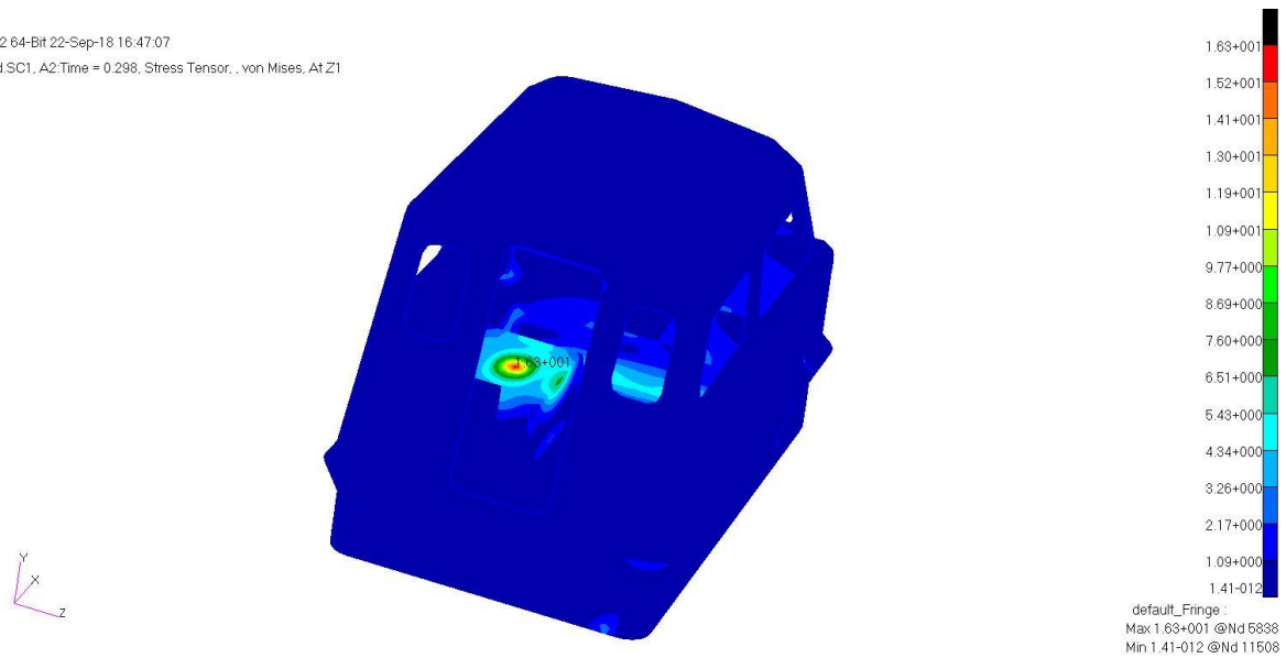
Figure 26. Cabin Stress Contour Plot at Z1: Port Seat Pedestal Node 5838
