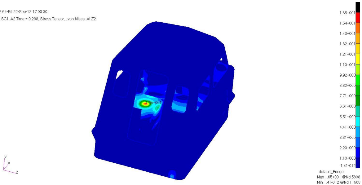
Figure 25. Cabin Stress Contour Plot at Z2: Port Seat Pedestal Node 5838
